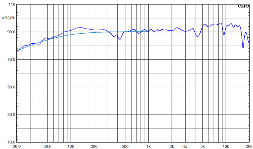
The frequency response above shows the measured anechoic axial sound pressure level using a standard IEC test baffle. Input 2.83v RMS, microphone distance 0.5m, SPL normalized to 1m value. The light blue line is the calculated low-frequency infinite baffle response from the parameters given in this datasheet. Impedance is measured in free space with a 1v input signal.
